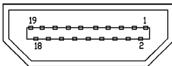
HDMI 19pin Connector
